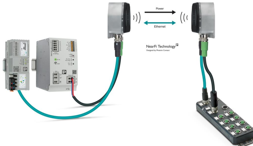
Figure 3 Example design for contact-free transmission of power and data between a controller and a decentral I/O device with Ethernet interface
