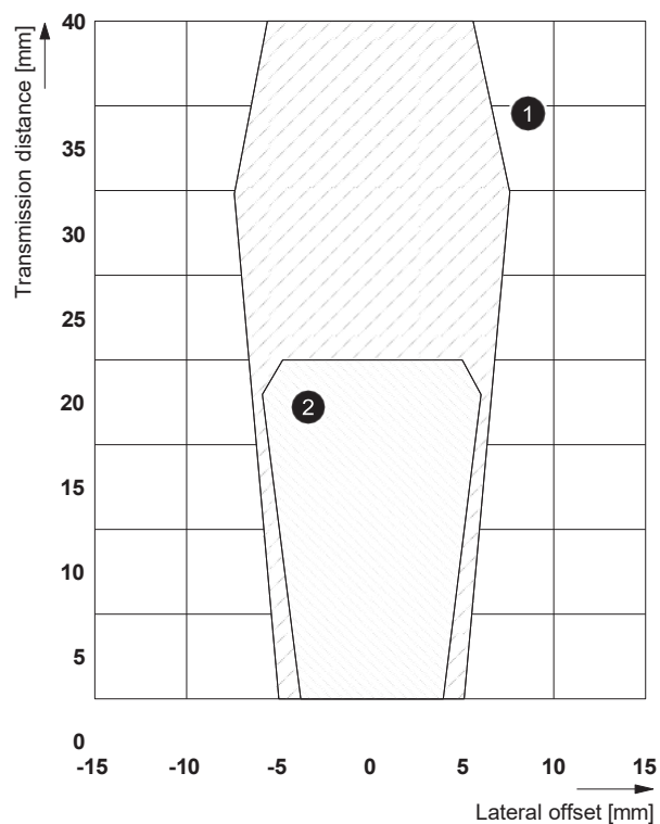
Figure 17 Transmission distance for lateral offset, NEARFI D...
