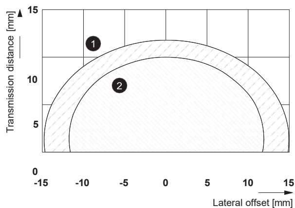
Figure 15 Transmission distance for lateral offset, NEARFI P...
