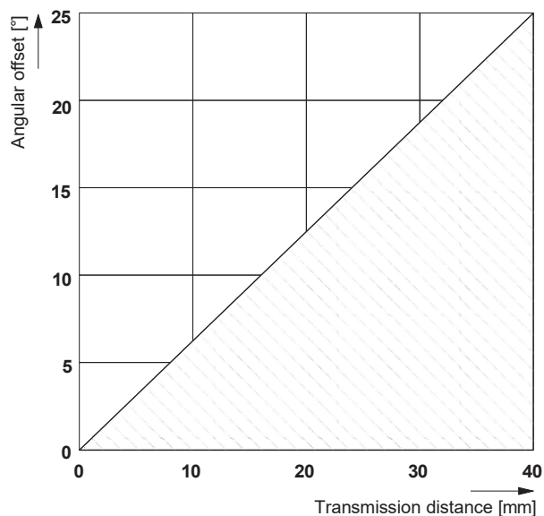
Figure 18 Transmission distance for angular offset, NEARFI D...
