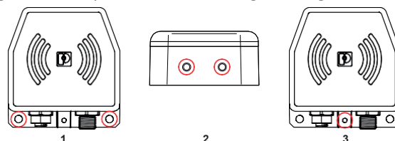
Figure 35 Options for functional grounding
