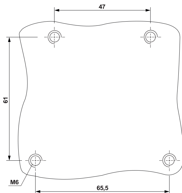
Figure 26 Drilling diagram
