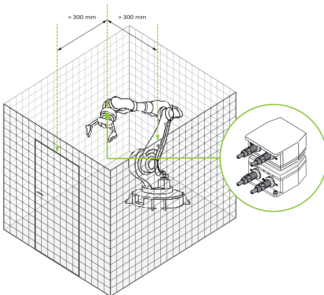
Figure 1 Industrial robots
