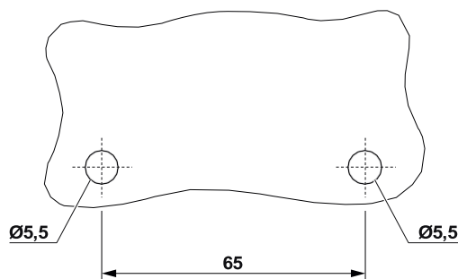
Figure 24 Drilling diagram
