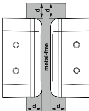
Figure 20 Metal-free area
