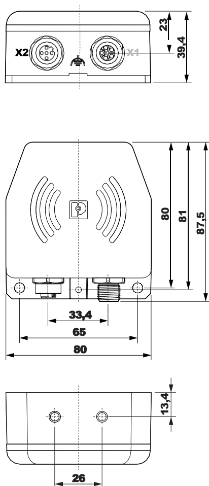
Figure 4 Housing dimensions
