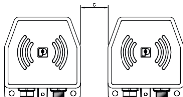
Figure 19 Minimum distance
