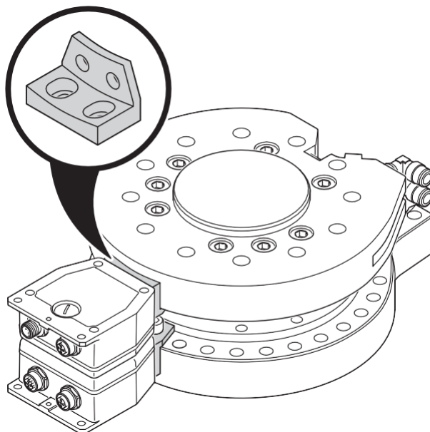
Figure 45 Installation example with external heatsink (processing head)
