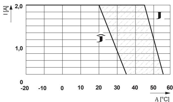
Figure 42 Derating curve
