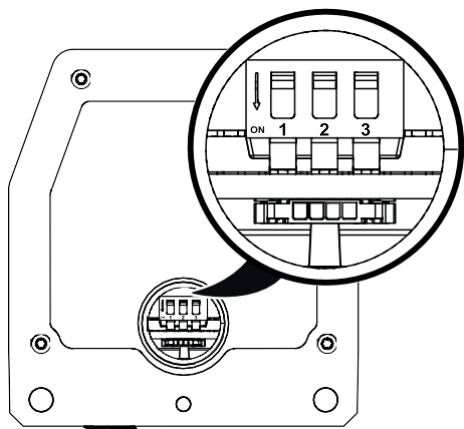
Figure 9 DIP switches
