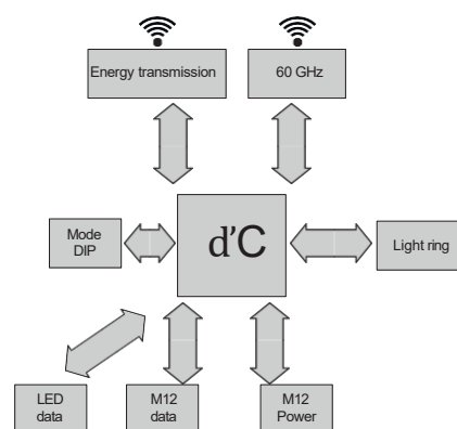
Figure 5 Basic circuit diagram of power and data couplers
