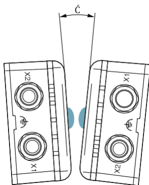
Figure 12 Angular offset
