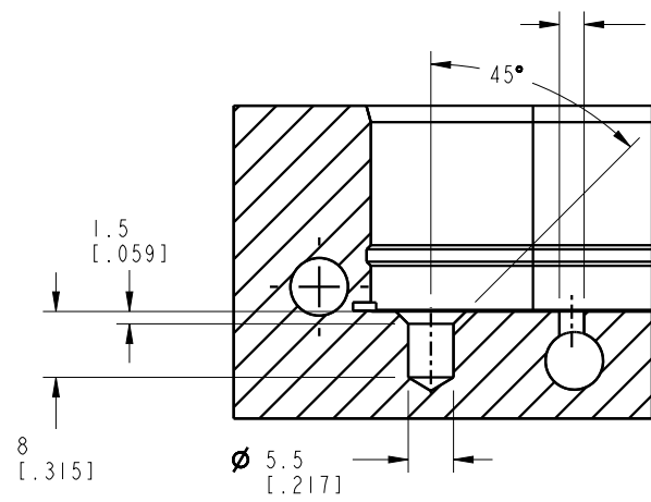
SECTION C-C
