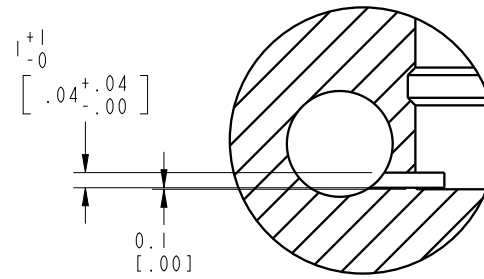
DETAIL Z
