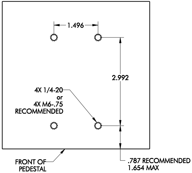
MOUNTING PATTERN FOR MODEL NO.56-0010-11
