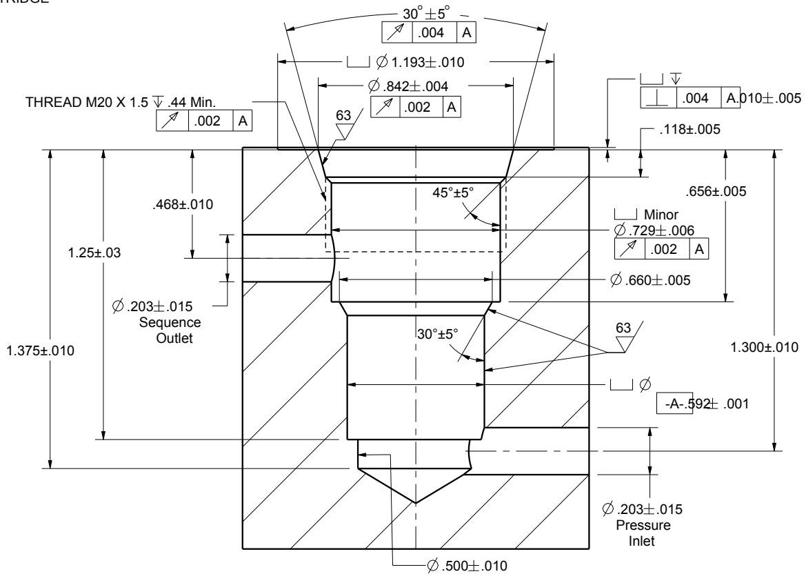
SEQUENCE VALVE CARTRIDGE CAVITY DIMENSIONS FOR MACHINING WITH PORT TOOL
