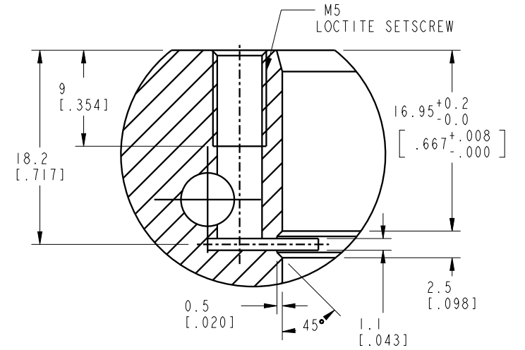
DETAIL Z
