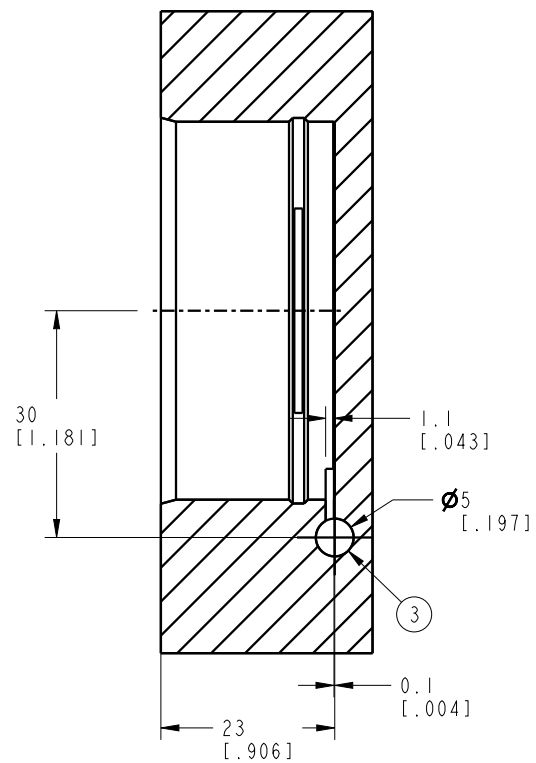
SECTION B-B
